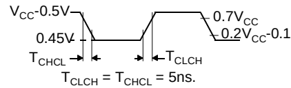
Figure 58. Clock Signal Waveform for I_{CC} Tests in Active and Idle Modes
