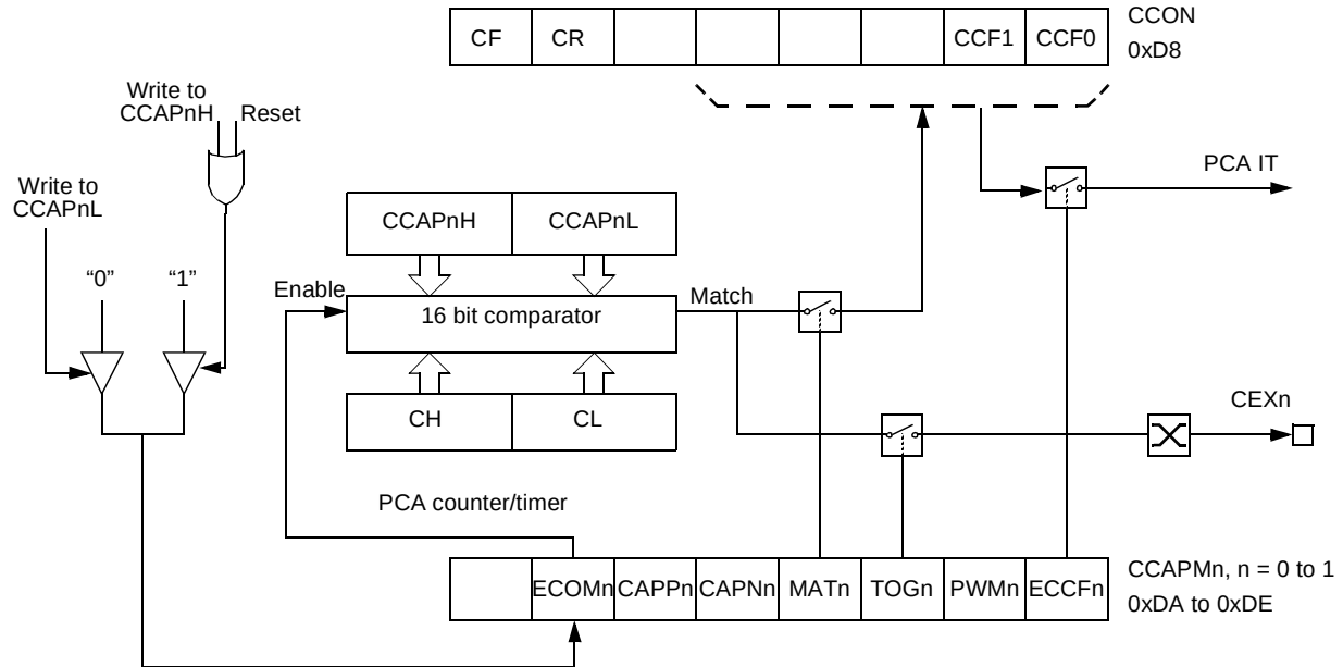
Figure 46. PCA High Speed Output Mode
